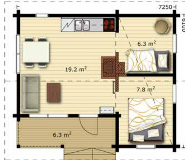
Alternative floor plan (without sauna)
