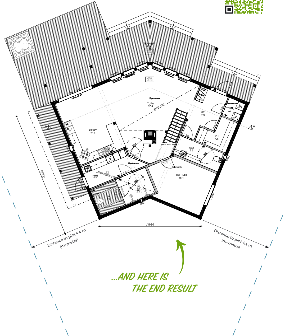
Nuuna 205 T2 variation 1st flr. floor plan.
