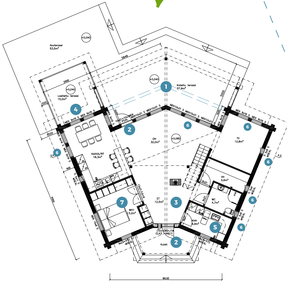
Nuuna 205 T2 1st flr. floor plan.
